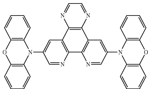
[Chemical Formula 8]
