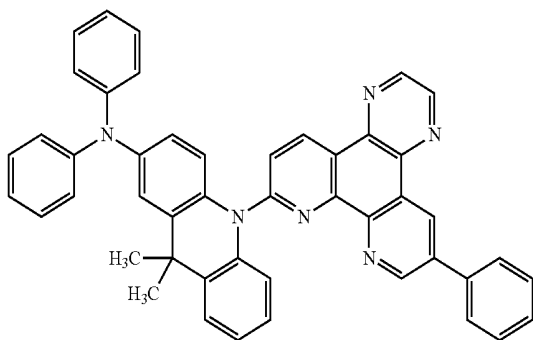
(Compound 96)
