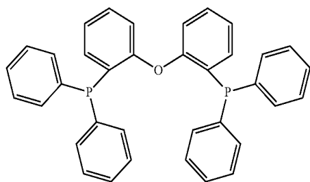
[Chemical Formula 132]
