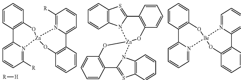
[Chemical Formula 143]
