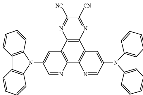
[Chemical Formula 33]
