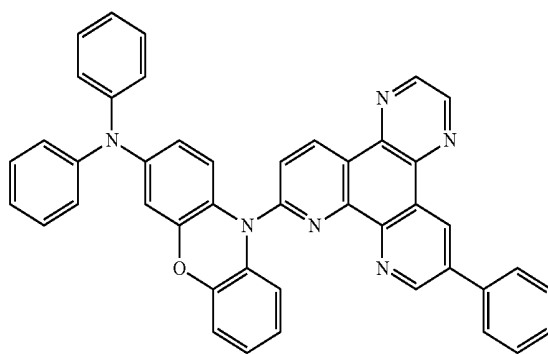
(Compound 93)
