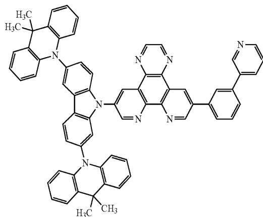
[Chemical Formula 91]
