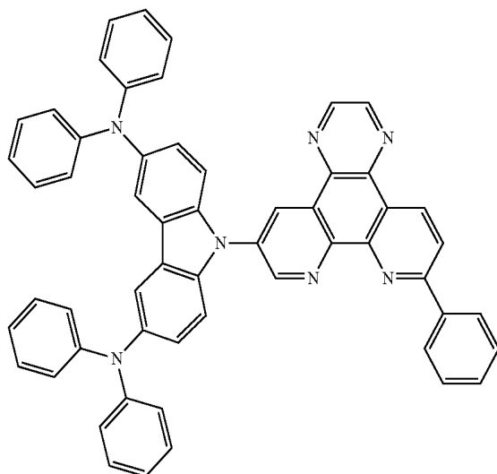
[Chemical Formula 115]
