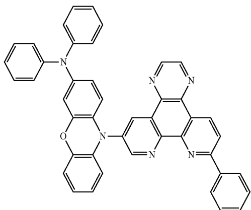
[Chemical Formula 101]
