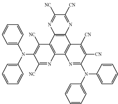
[Chemical Formula 34]
