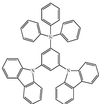
[Chemical Formula 131]
