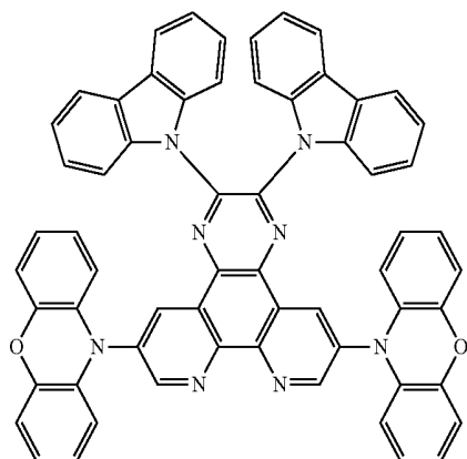
[Chemical Formula 36]
