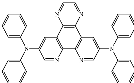
[Chemical Formula 11]
