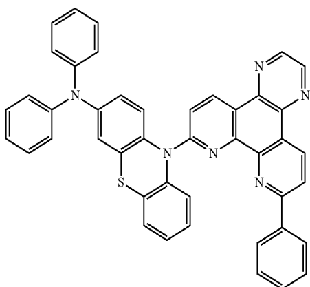
[Chemical Formula 101]
