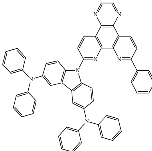
[Compound Formula 114]
