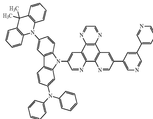
[Chemical Formula 92]
