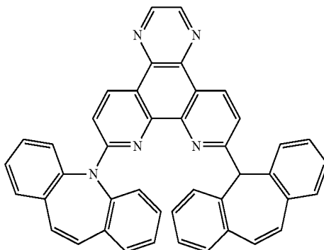
[Chemical Formula 13]
