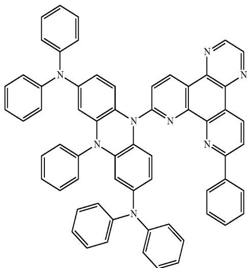
[Compound Formula 113]
