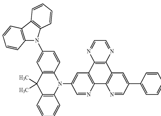
(Compound 109)
