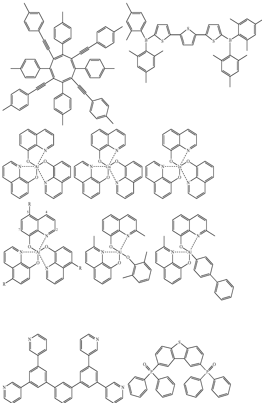
[Chemical Formula 142]
