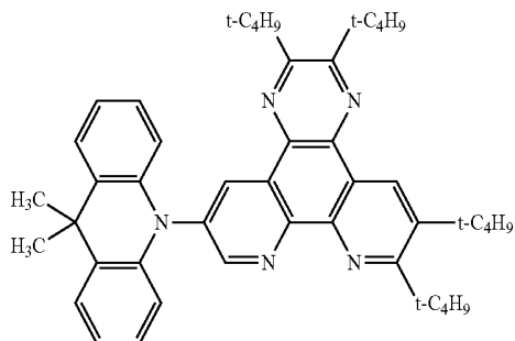
[Chemical Formula 88]
