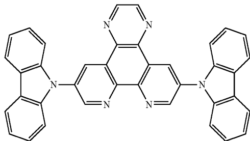
[Chemical Formula 10]
