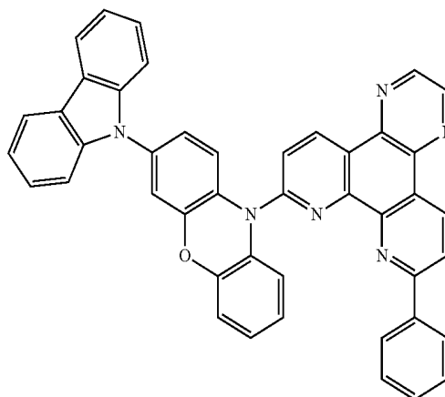
(Compound 107)
