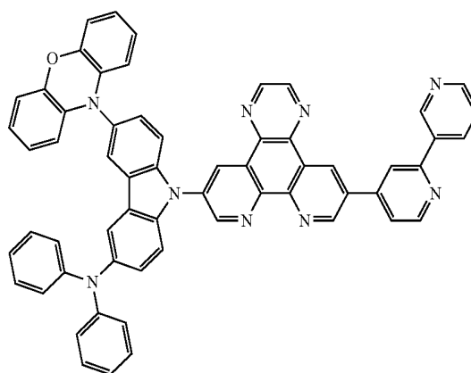
(Compound 85)
