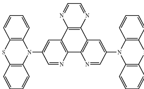
[Chemical Formula 9]
