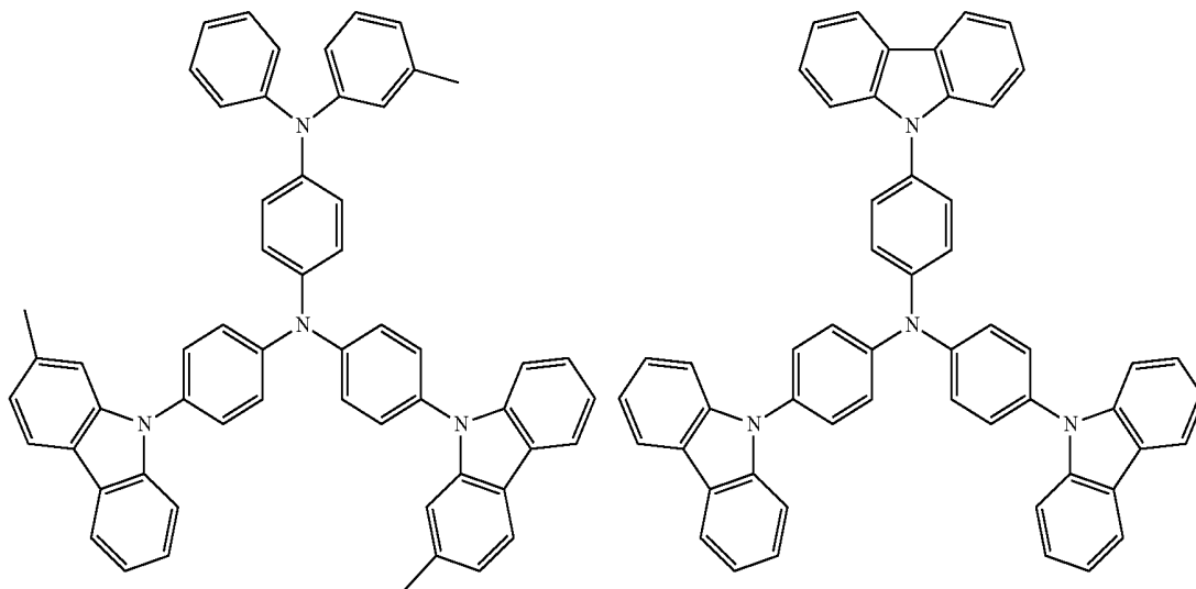
[Chemical Formula 136]
