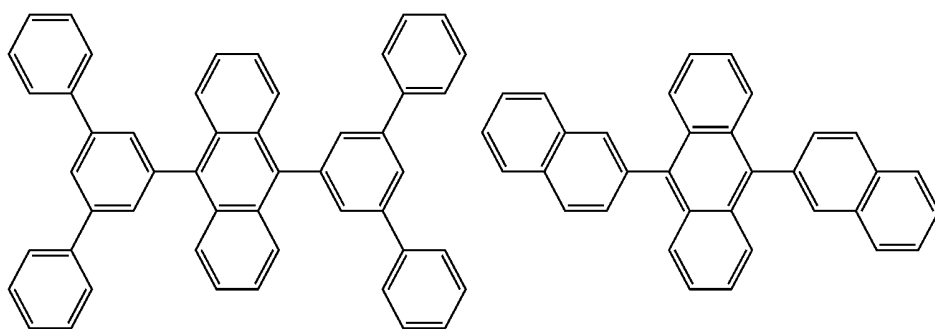
[Chemical Formula 131]
