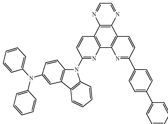
(Compound 97)
