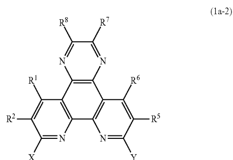
[Chemical Formula 5]
