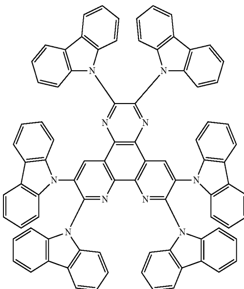
(Compound 8)
