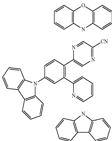
[Chemical Formula 36]
