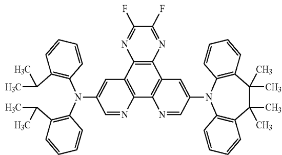
(Compound 28)
