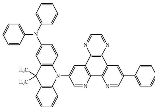
(Compound 95)
