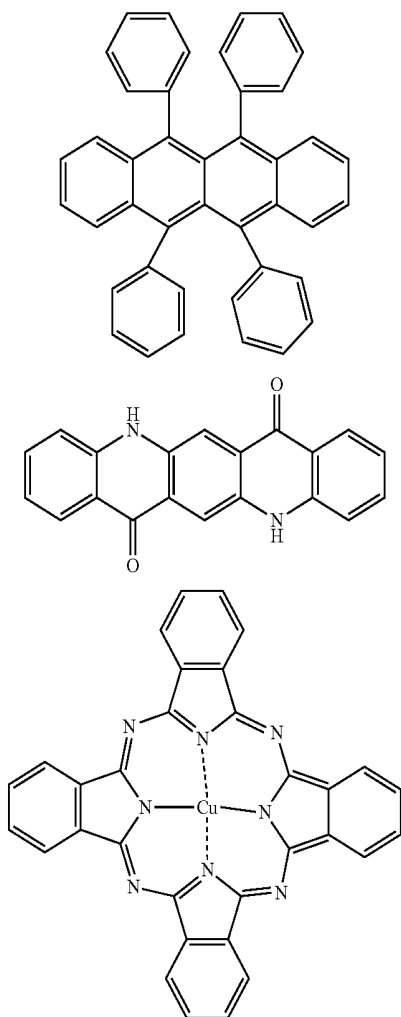
[Chemical Formula 146]
