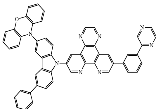
(Compound 84)
