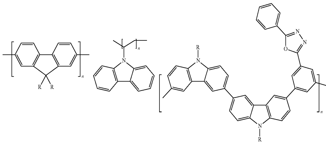
[Chemical Formula 132]
