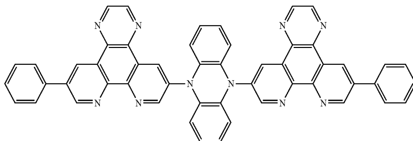
[Chemical Formula 89]
