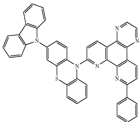
[Chemical Formula 115]
