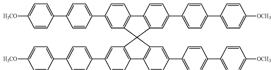
[Chemical Formula 128]
