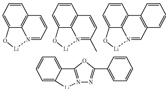
[Chemical Formula 145]
